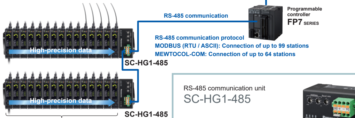
Connection of 1 master unit and up to 14 slave units*
