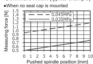
<Downward mount (typical example)>
